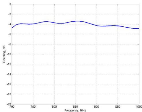
Coupling to internal modem antenna
